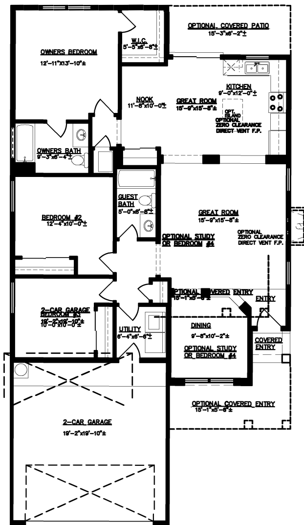
OPTIONAL LUXURY OWNERS BATH (OWNERS BEDROOM BECOMES SMALLER)
