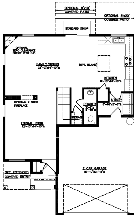
DOWNSTAIRS FLOORPLAN
