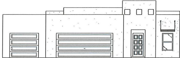
FRONT ELEVATION
