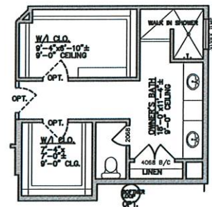
⑦ OPT. OWNER'S BATH W/ WALK IN SHOWER
