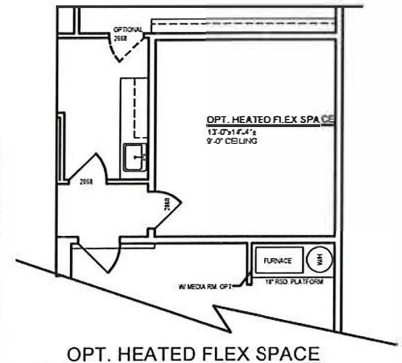
OPT. HEATED FLEX SPACE
