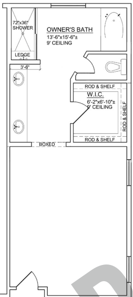
OPT. OWNER'S BATH #1
