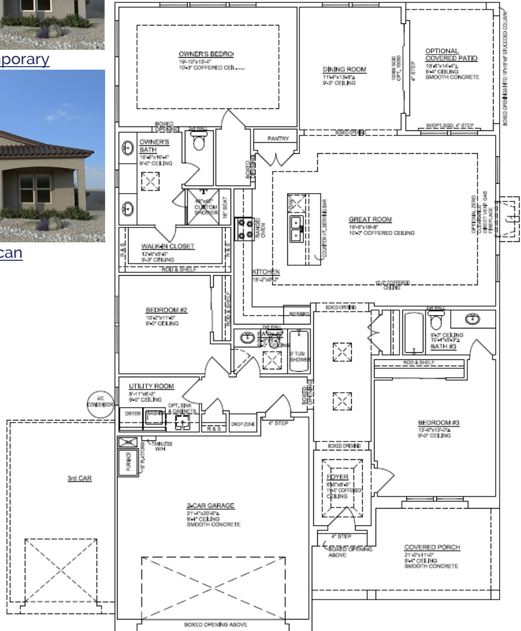
FLOOR PLAN
