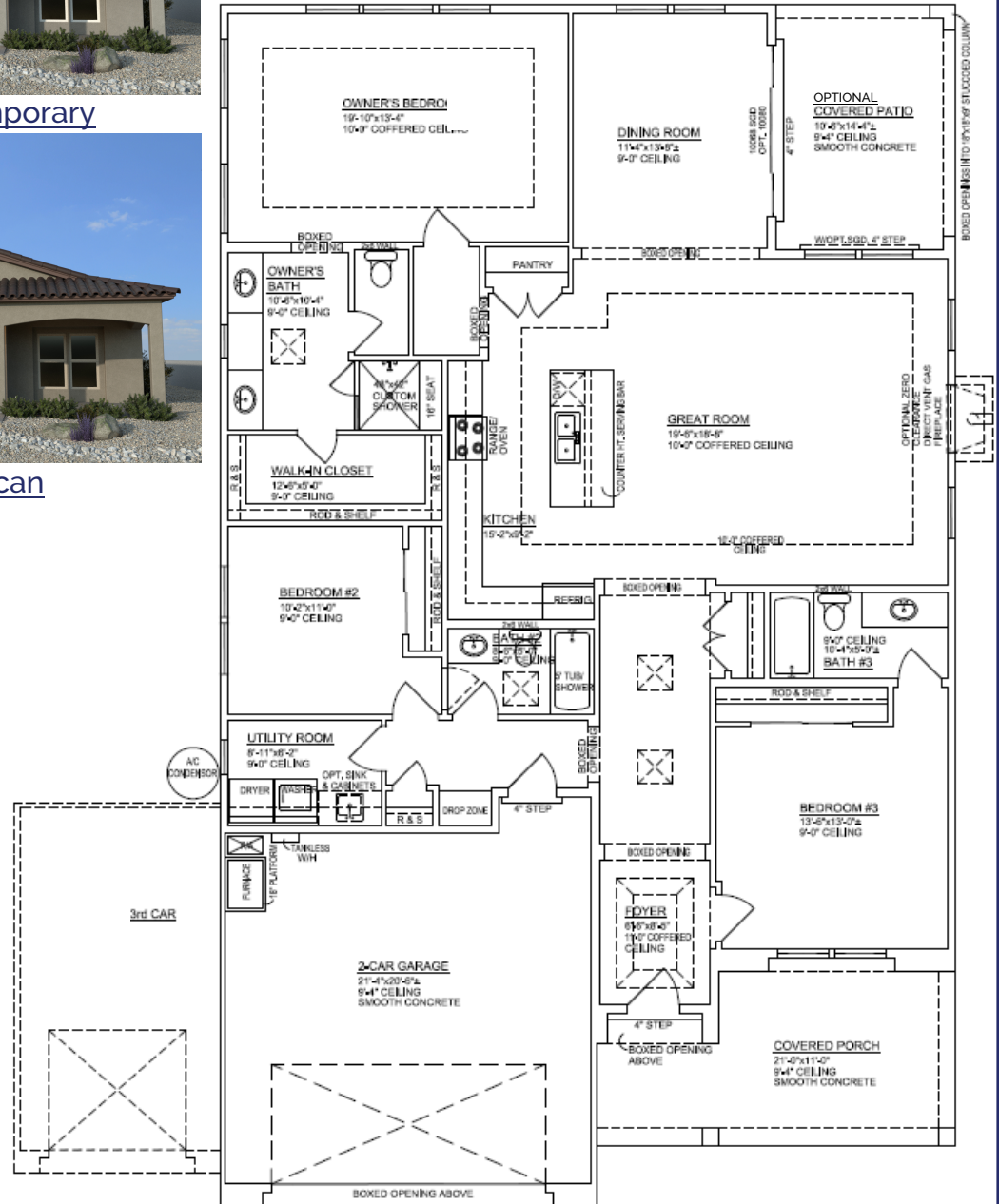
FLOOR PLAN
