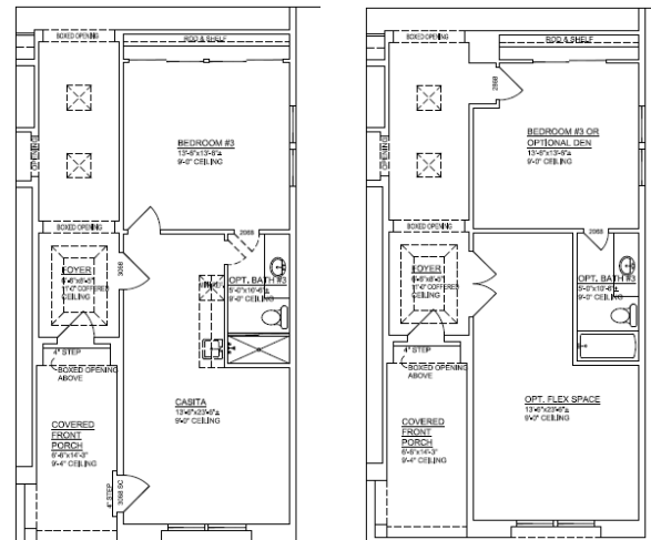
FLOOR PLAN - W/ OPT. CASITA
