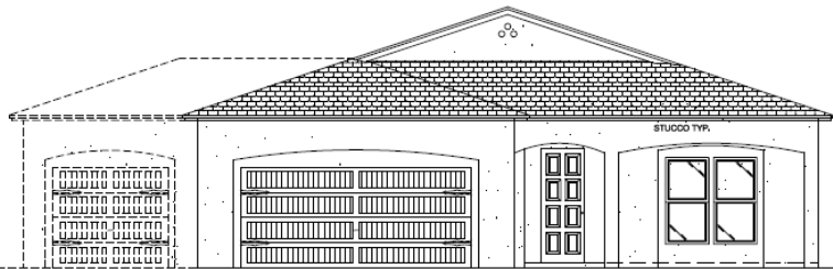
FRONT ELEVATION - STD., TUSCAN
