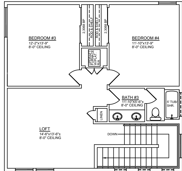
UPSTAIRS FLOOR PLAN
